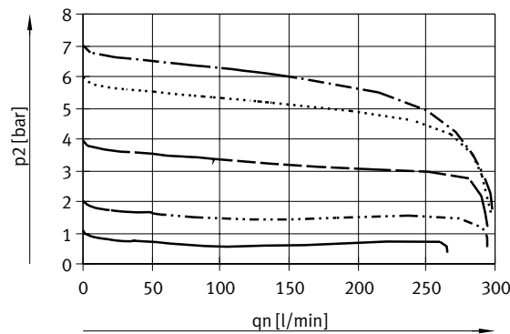
Standard flow rate q_n as a function of output pressure p_2 ( p_1 = 8 \text{ bar} ) MS2-LR-QS6-B
