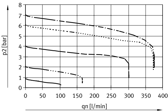
Standard flow rate q_n as a function of output pressure p_2 ( p_1 = 10 \text{ bar} ) MS2-LR-M5-B
